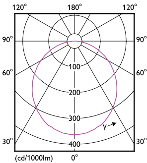
Downlight 59466 MESON 150 65K WH Recessed-LDD
