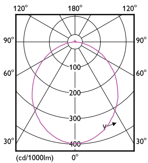
Downlight 59448 MESON 105 30K WH Recessed TR-LDD
