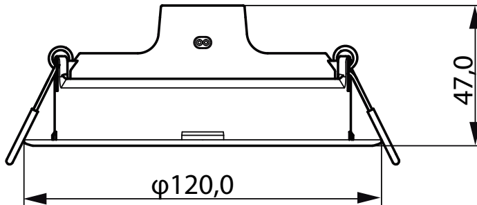
59448 MESON 105 7.5W 30K WH recessed TR
