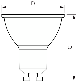
ESS LEDspots 50W GU10 830 36D ND TR
