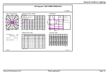
LED Lamps, CorePro LEDcapsuleLV 1-10W G4 827
